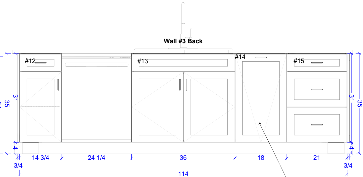
B Island Front Scale : 3/4" = 1'
