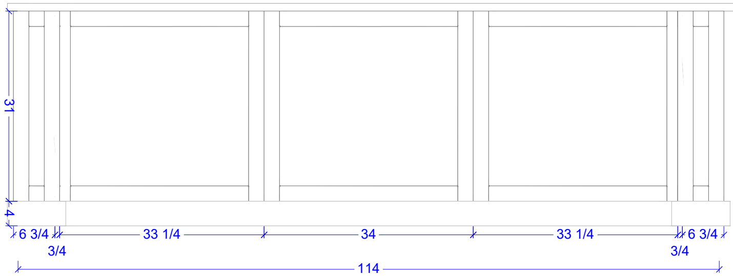
C Island Back Scale : 3/4" = 1'
