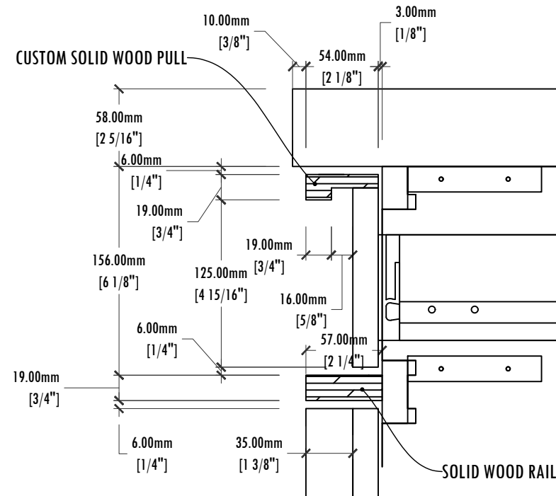
C LAUNDRY - SINK CABINET PULL DETAIL SCALE: 1:4 ARCH. REF.:
