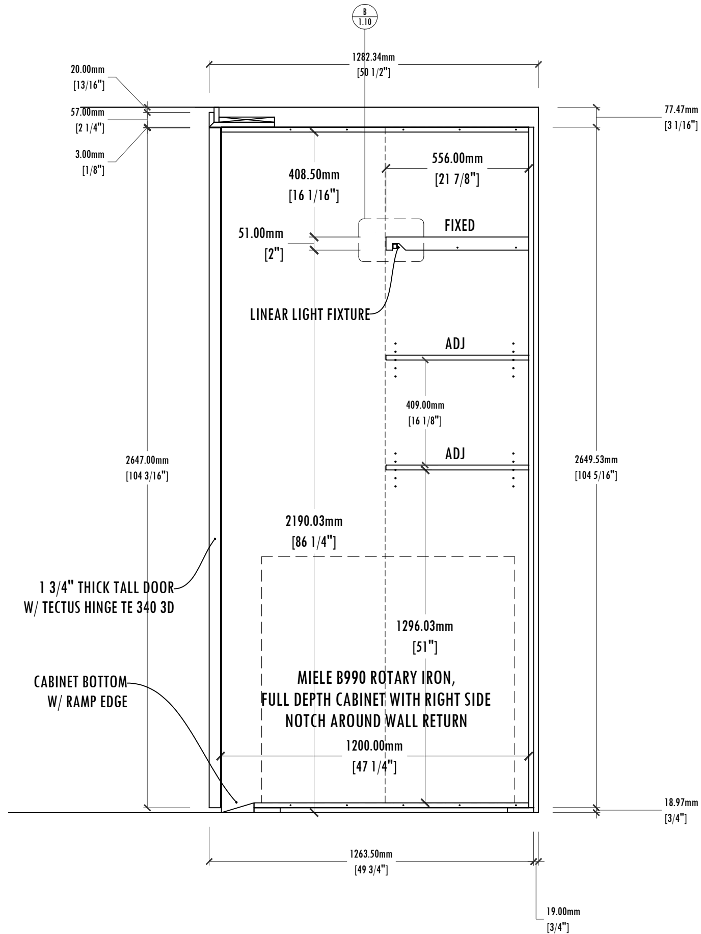
A LAUNDRY - SECTION SCALE: 1:15 ARCH. REF.:
