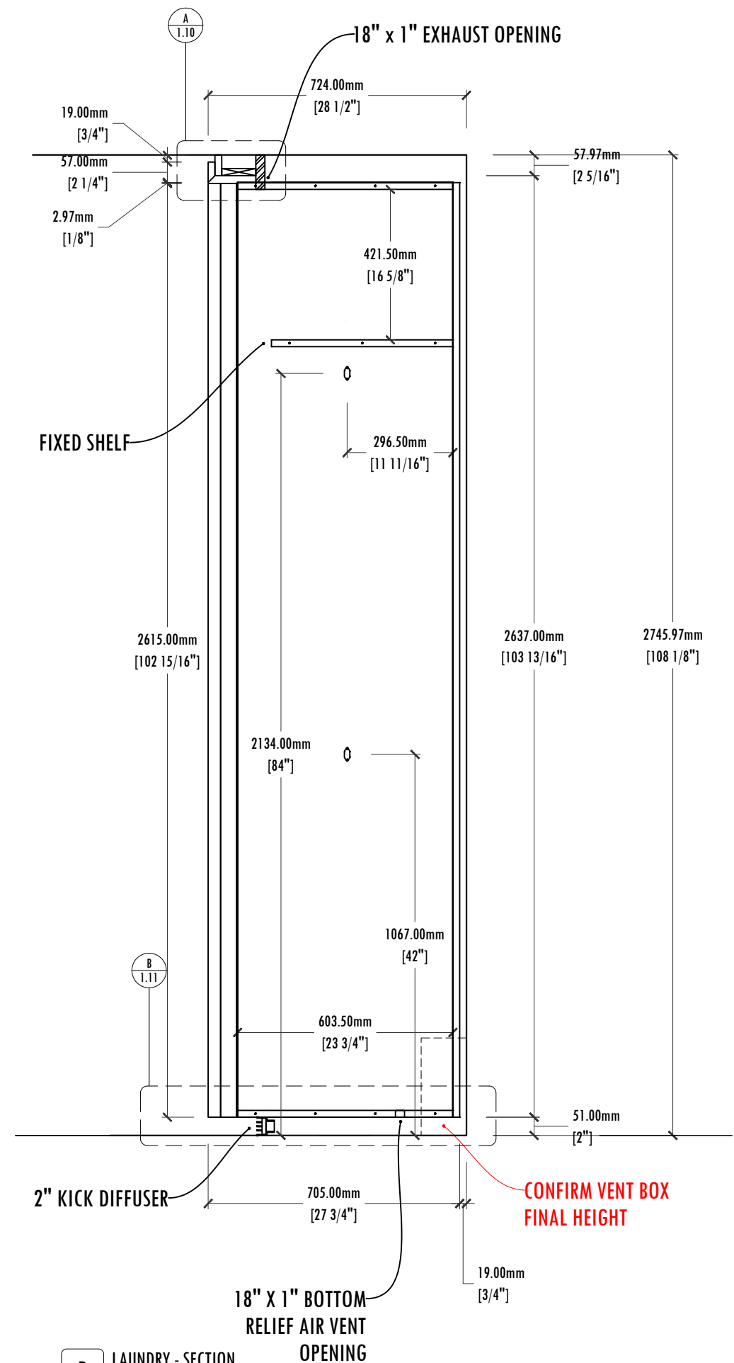
B LAUNDRY - SECTION SCALE: 1:15 ARCH. REF.:
