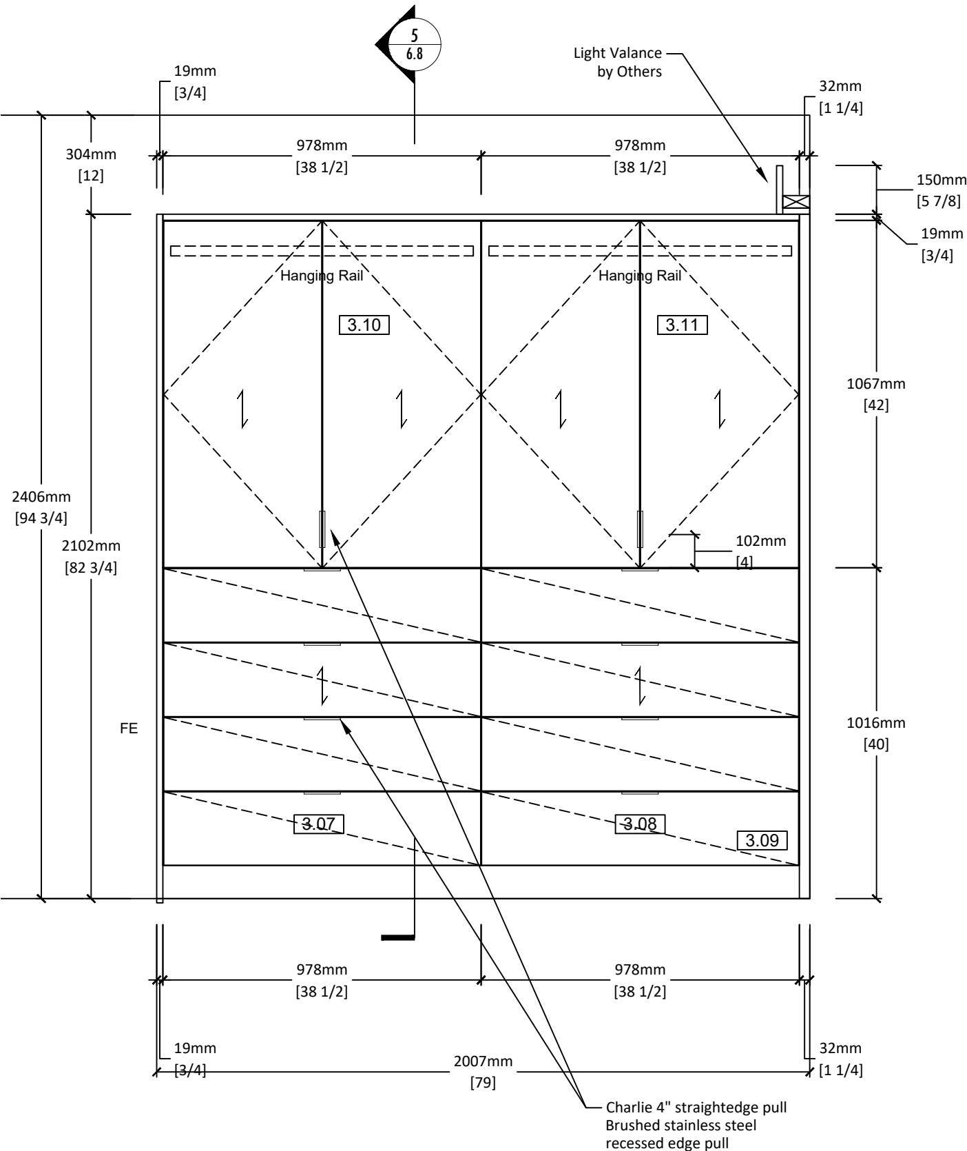
C BEDROOM 1 - ELEVATION SCALE: 1:16 ARCH. REF.:
