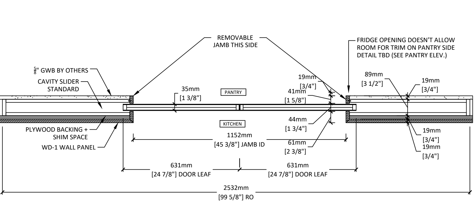
D1 POCKET DOOR - PLAN DETAIL SCALE: 1:12 ARCH. REF.:
