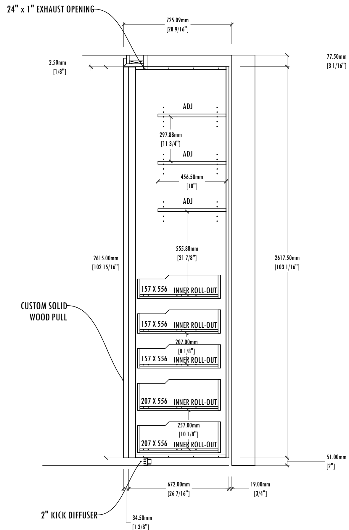
B LAUNDRY - SECTION SCALE: 1:15 ARCH. REF.:
