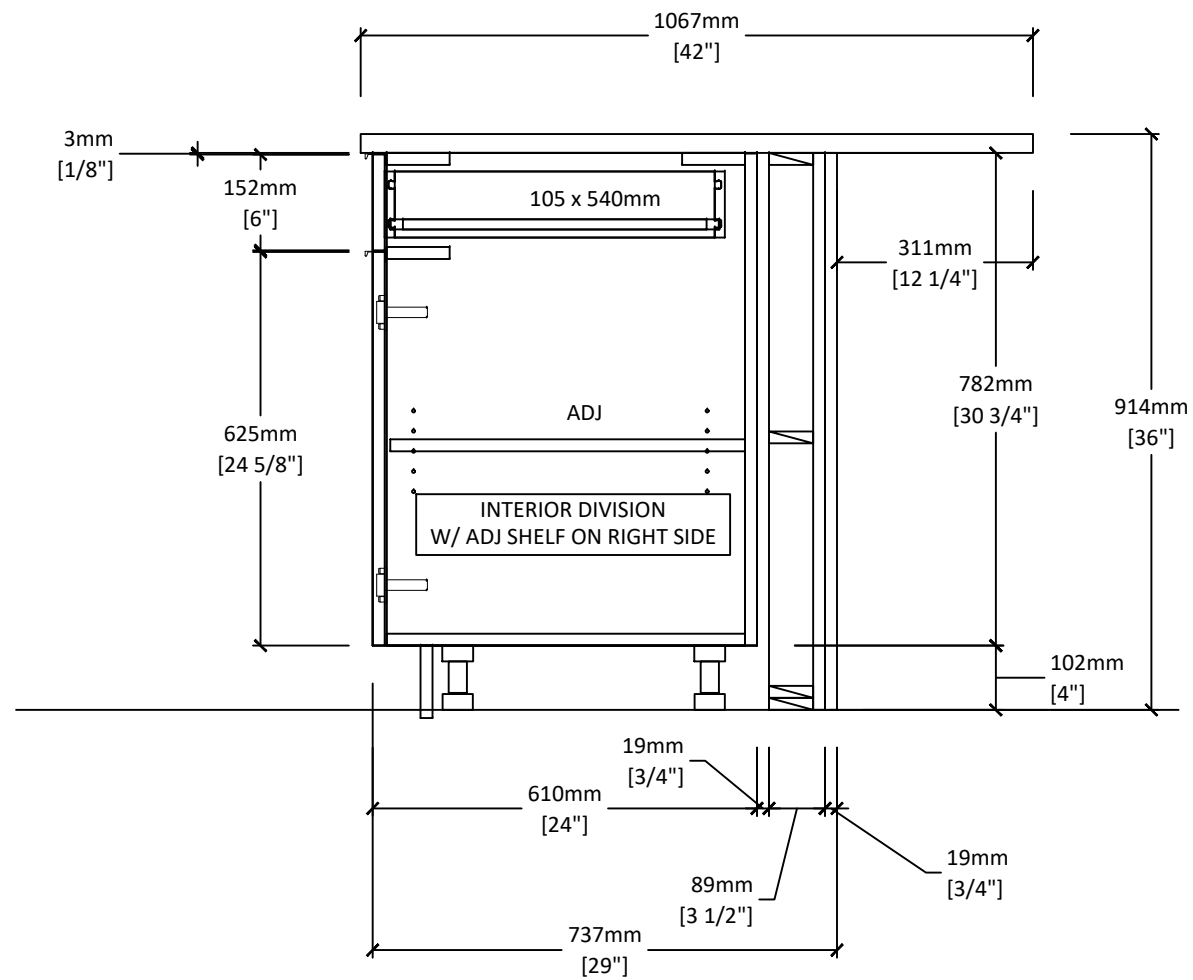
1 KITCHEN- SINK CABINET SECTION SCALE: 1:12 ARCH. REF.:
