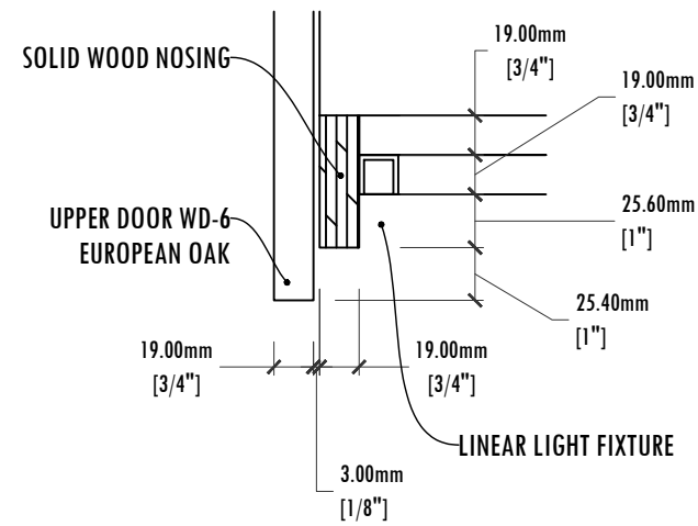
A LAUNDRY - UPER CABINET PULL AND LIGHT DETAIL SCALE: 1:4 ARCH. REF.:
