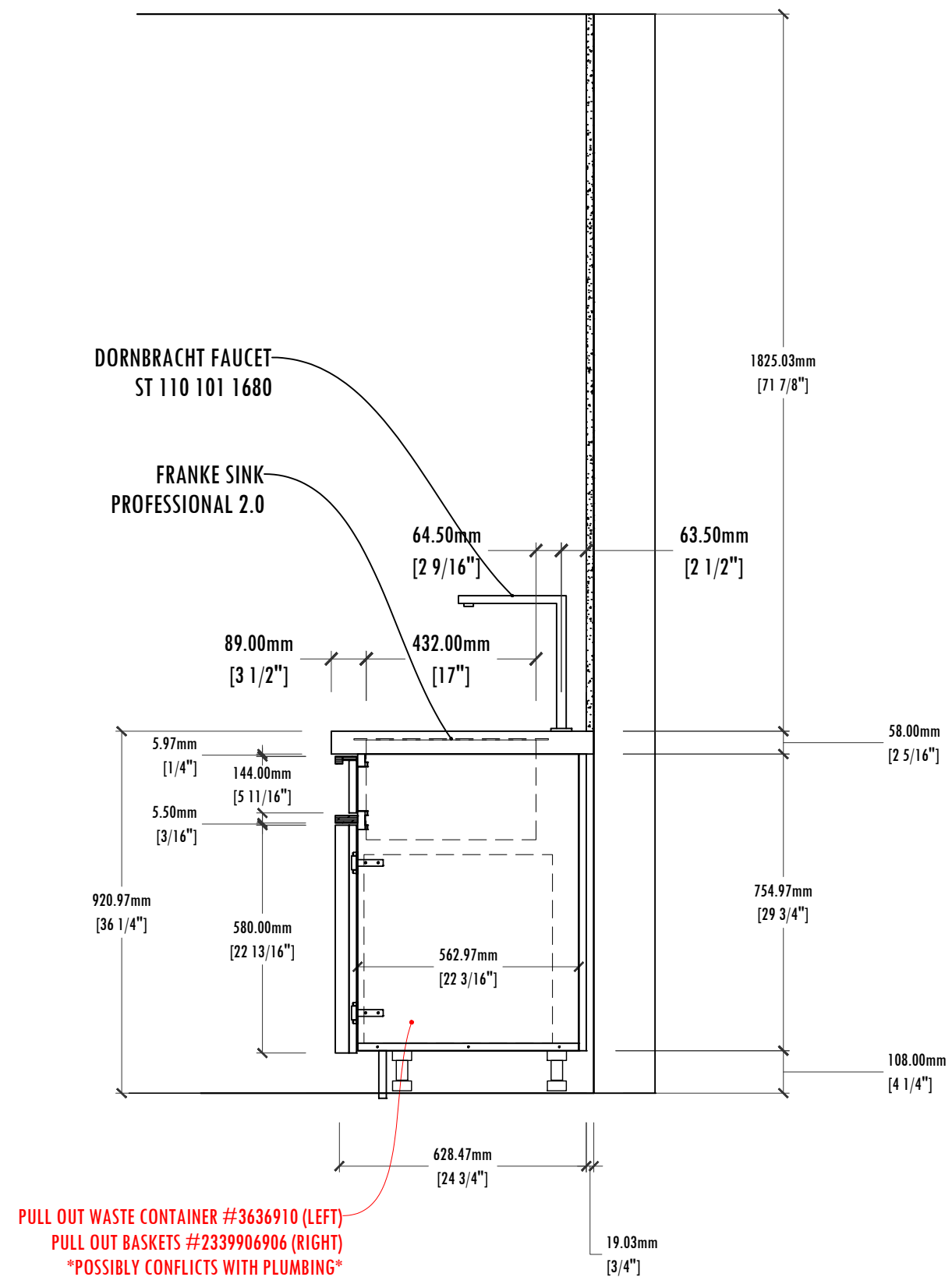
B LAUNDRY - SECTION SCALE: 1:15 ARCH. REF.:
