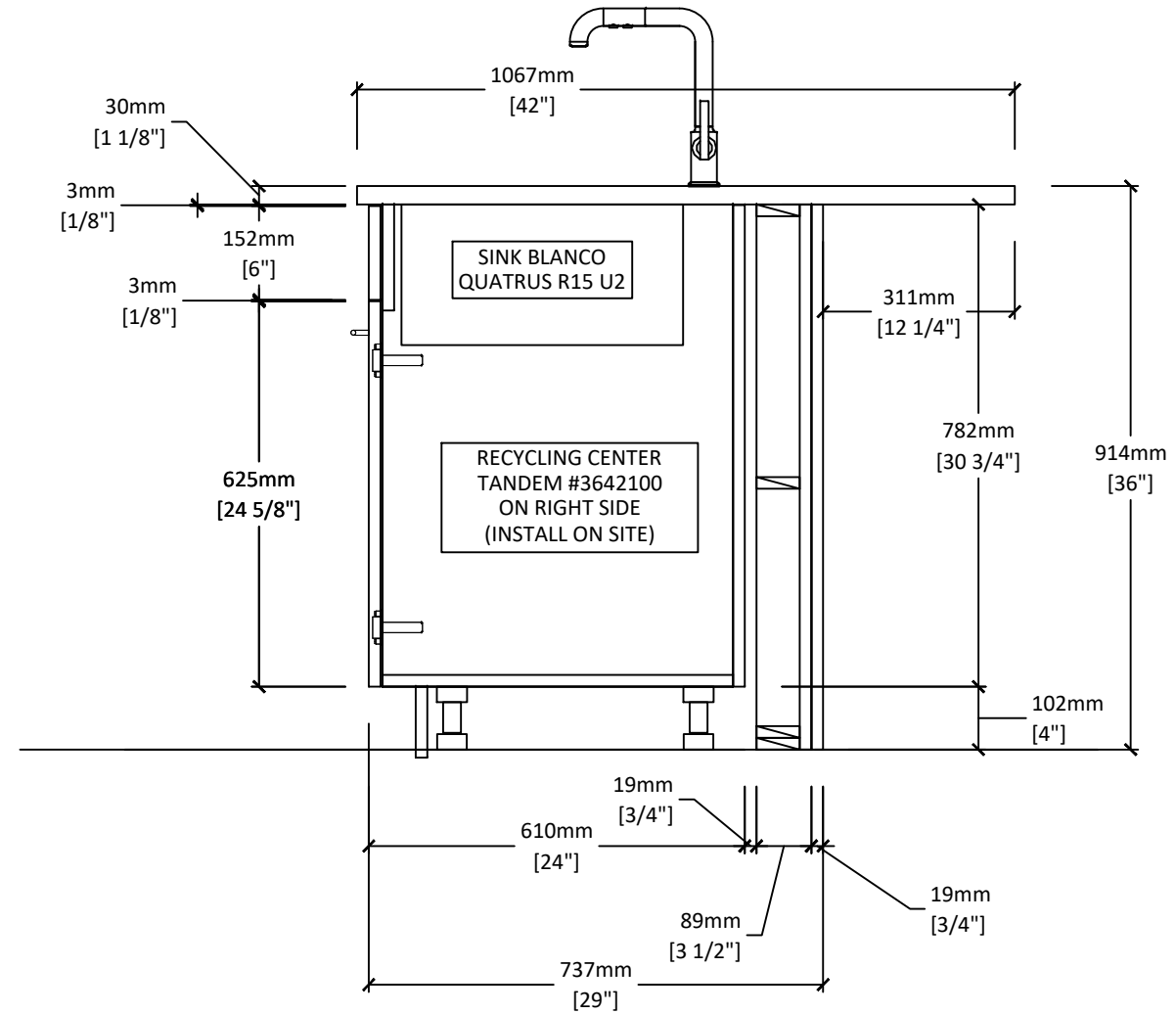
2 KITCHEN- SINK CABINET SECTION SCALE: 1:12 ARCH. REF.:
