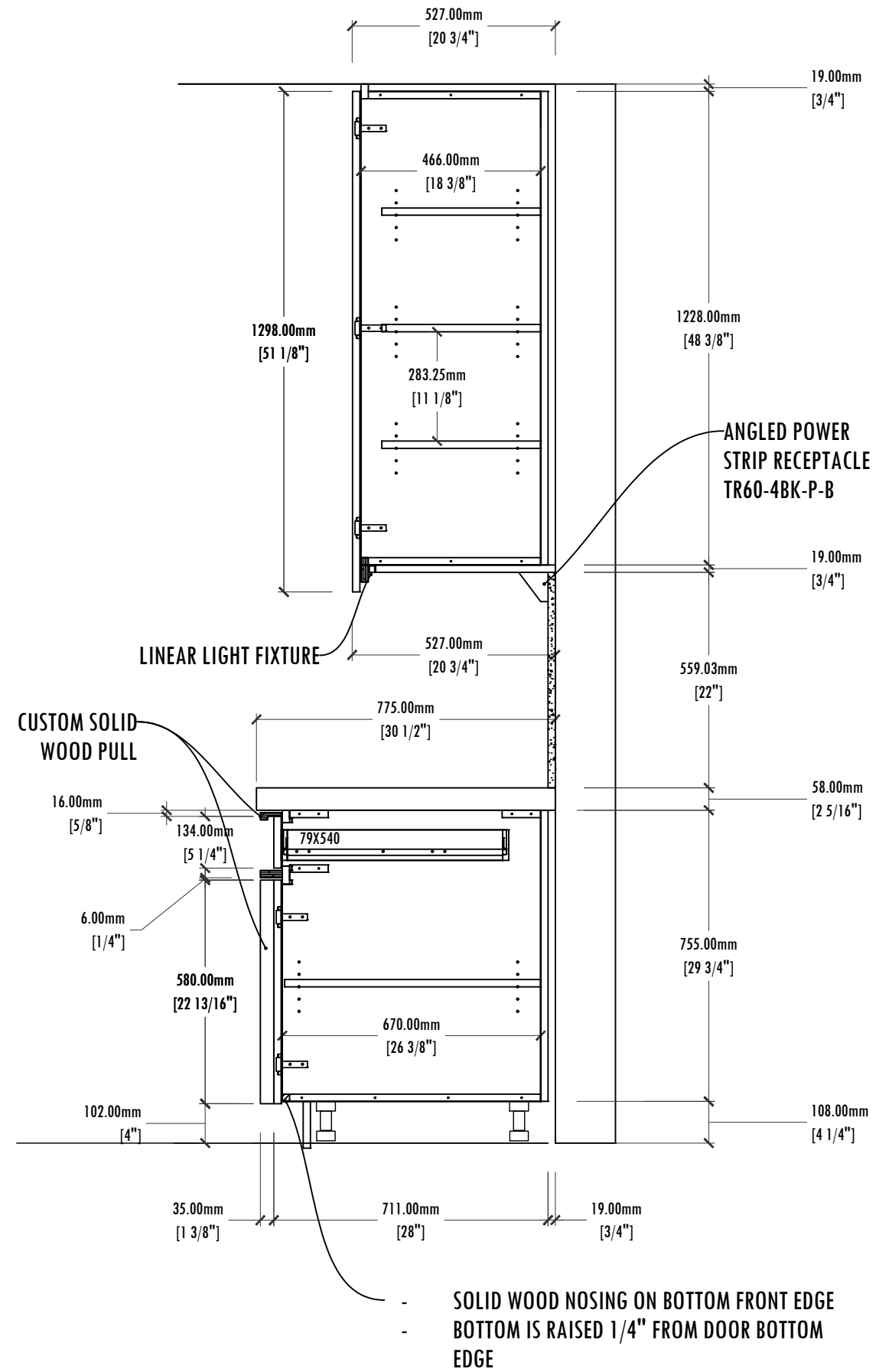
B LAUNDRY - SECTION SCALE: 1:15 ARCH. REF.:
