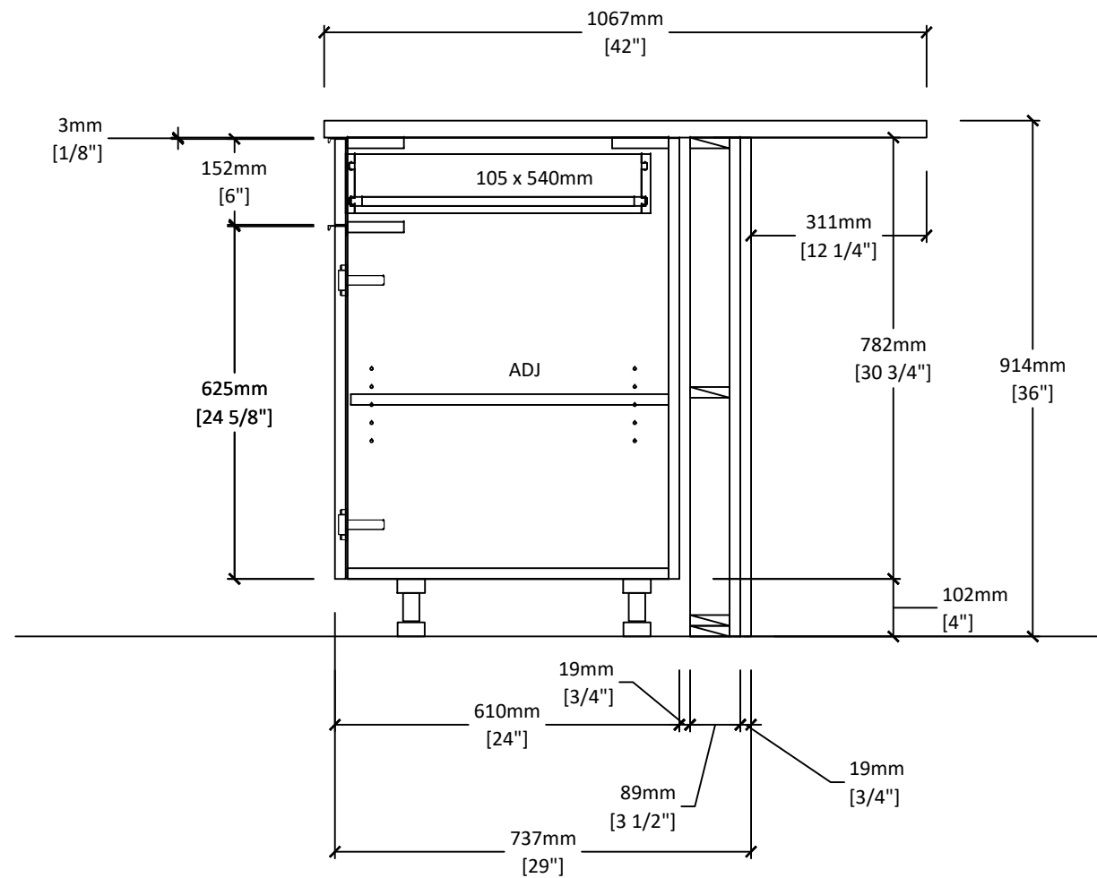
1 KITCHEN- SINK CABINET SECTION SCALE: 1:12 ARCH. REF.:
