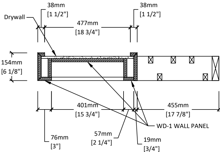
D4 CHARGING CUBBY - PLAN SECTION DETAIL SCALE: 1:12 ARCH. REF.:
