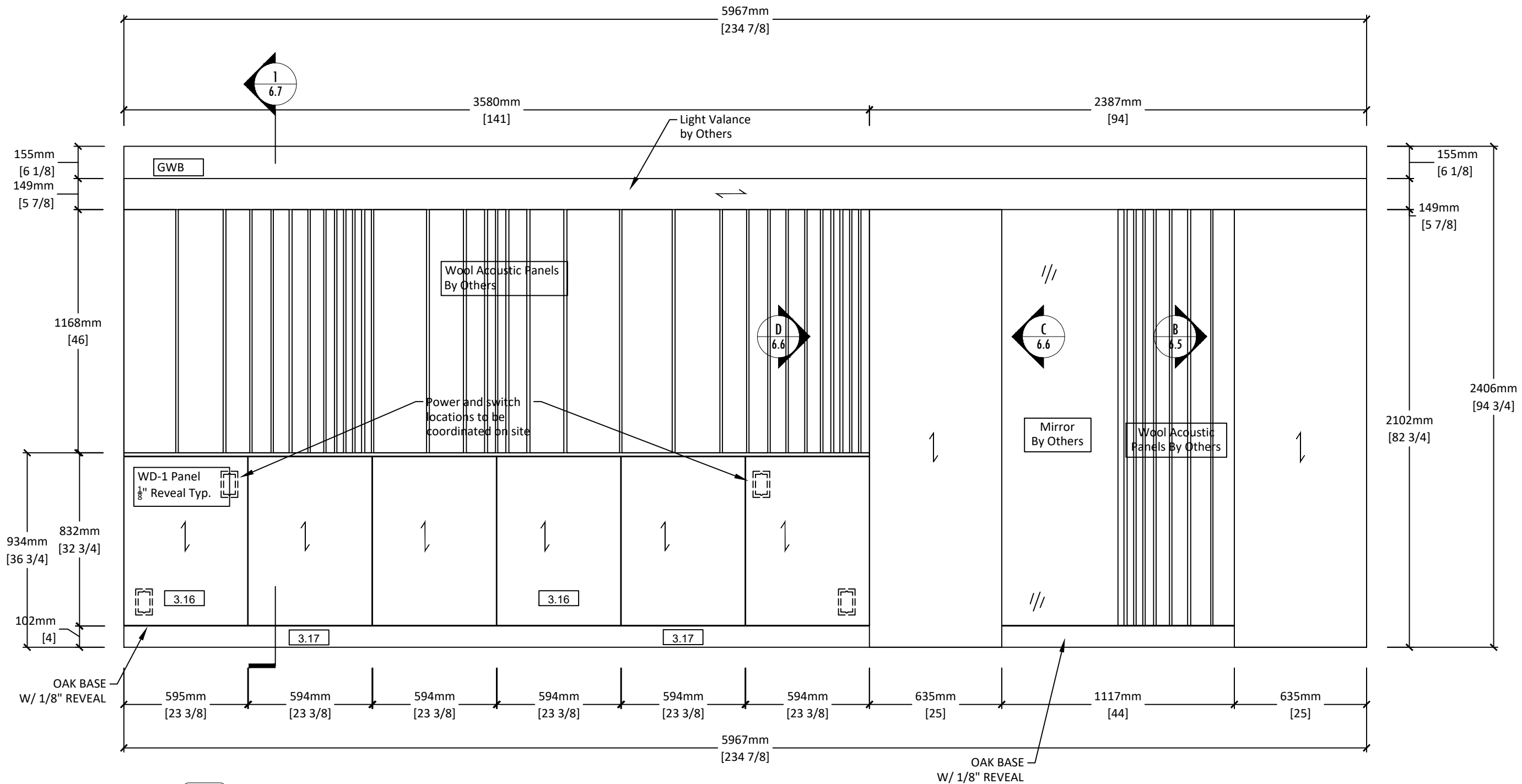
A BEDROOM 1 - ELEVATION SCALE: 1:20 ARCH. REF.:
