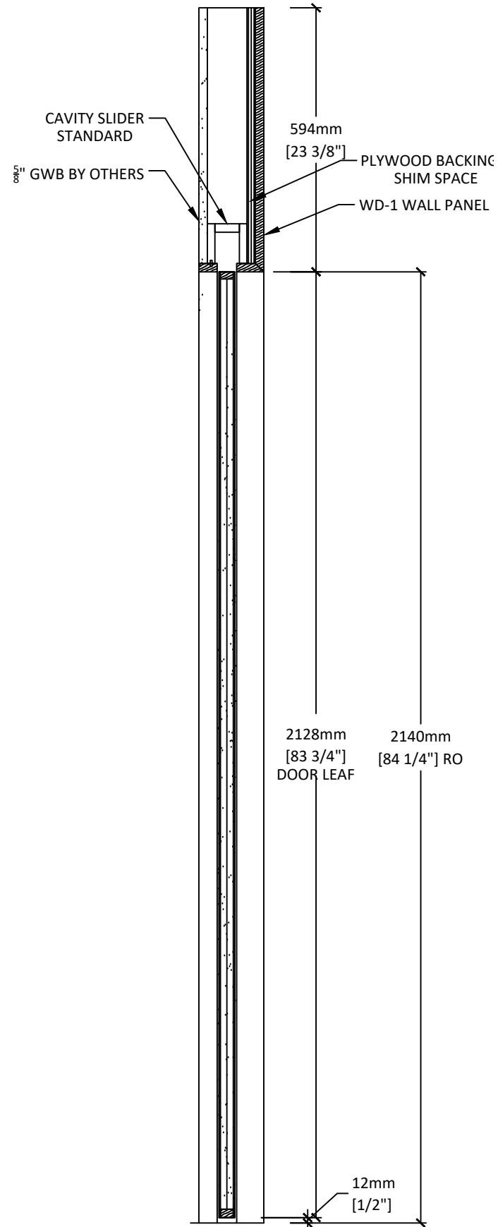
D2 POCKET DOOR - SECTION DETAIL SCALE: 1:12 ARCH. REF.:
