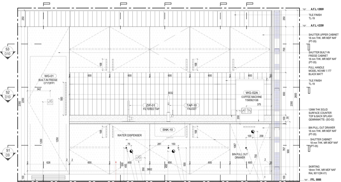
ELEVATION A SCALE-1:10
