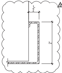
2 MTL CASING 1'-0" = 1'-0"
