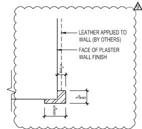
7 MTL CASING 1'-0" = 1'-0"
