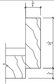
3 WD CASING 1'-0" = 1'-0"
