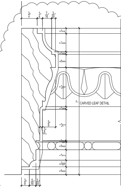
9 WD CASING 1'-0" = 1'-0"
