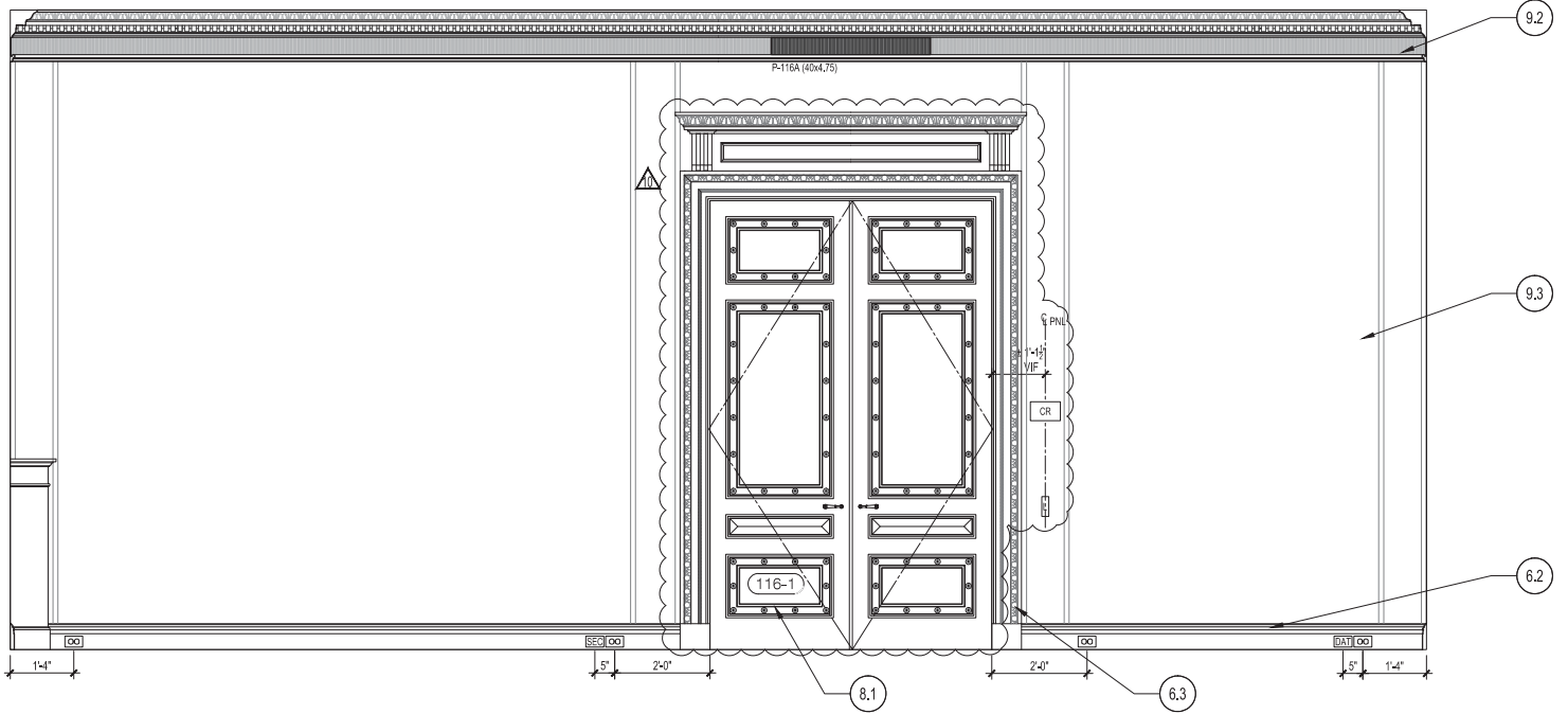
1 116/DINING ROOM 1/2" = 1'-0"
