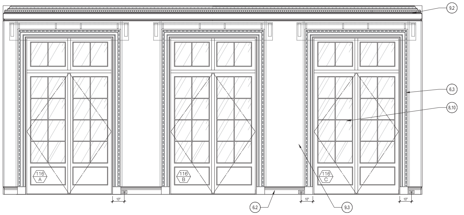
2 116/DINING ROOM 1/2" = 1'-0"
