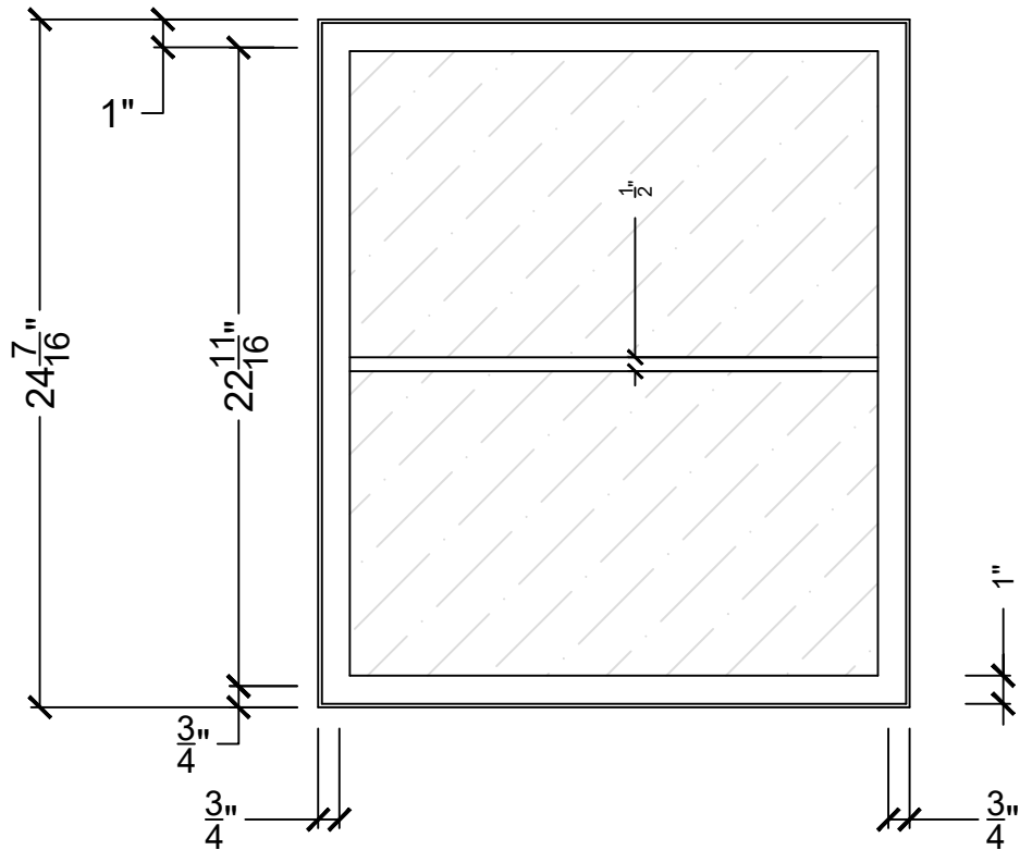
Elevation View Reference Only
