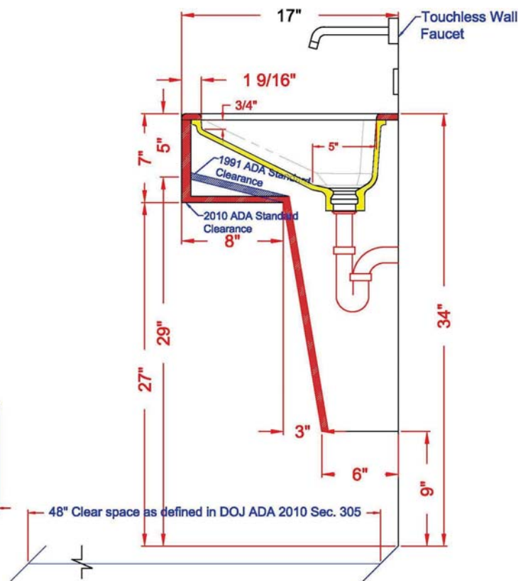
Section B-B
