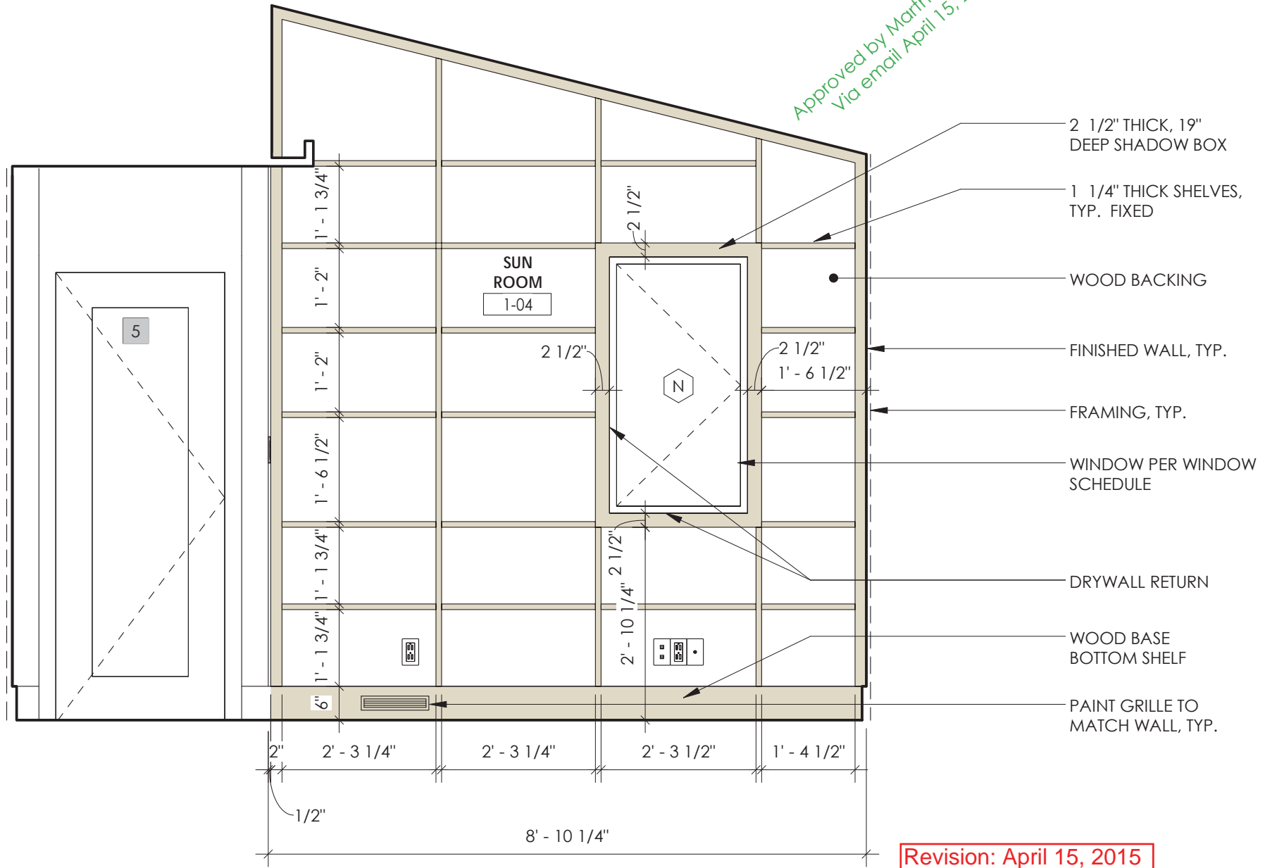
2 CABINERY PACKAGE - MAIN HOUSE - SUN ROOM - EAST ELEVATION 1/2" = 1'-0"
