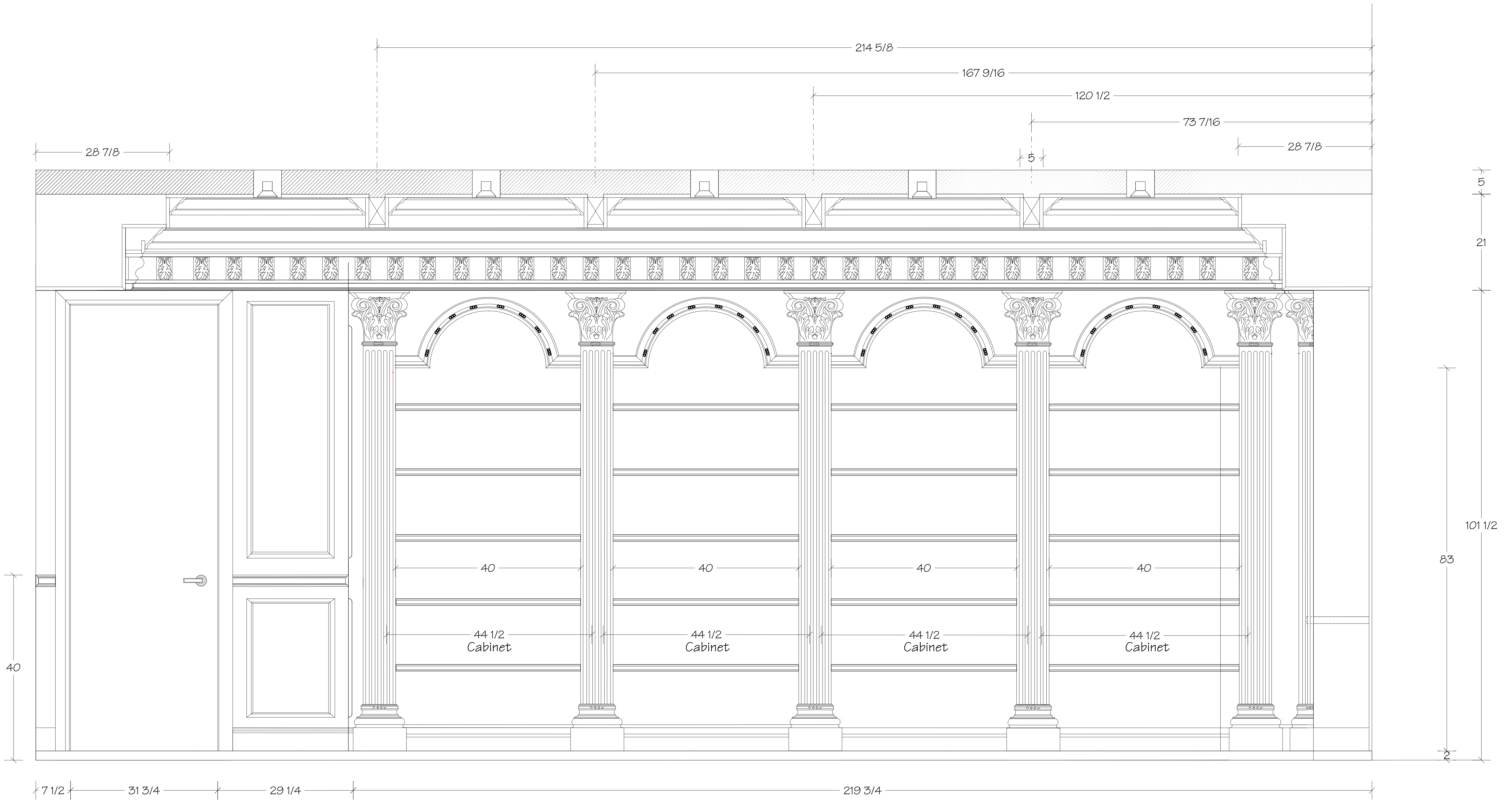
RODS OFFICE Elevation D
