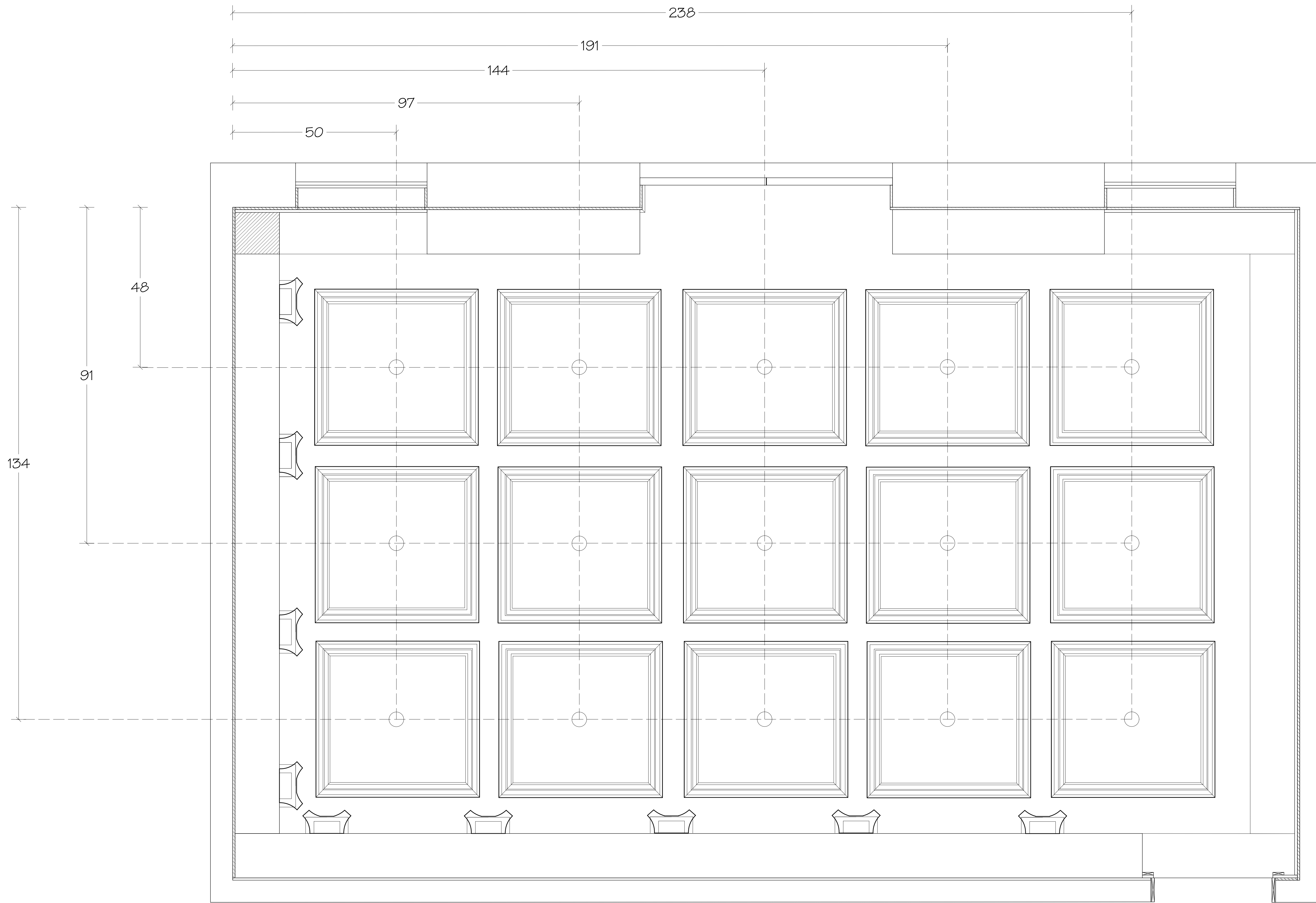
RODS OFFICE Ceiling Light Location
