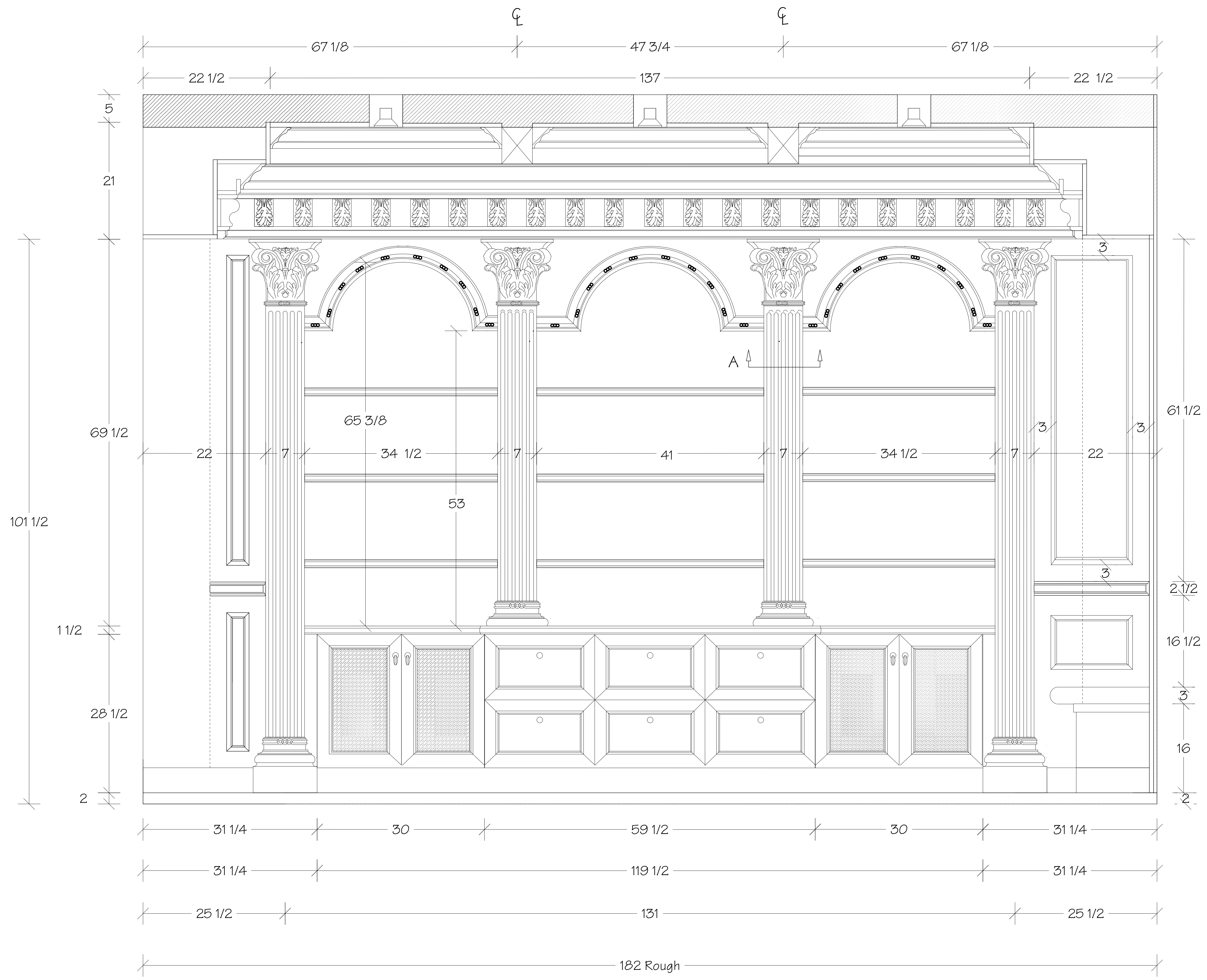
RODS OFFICE Elevation A
