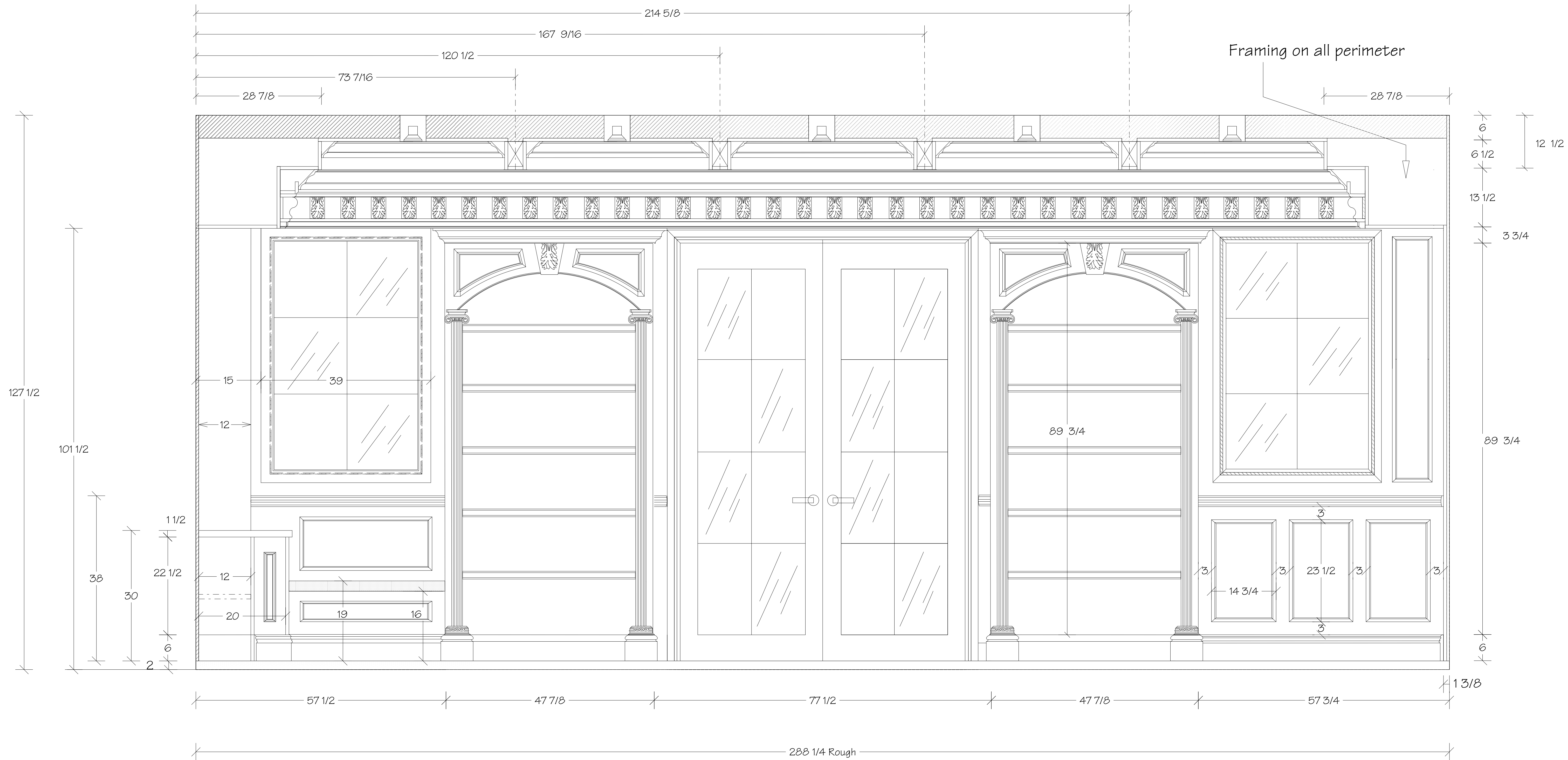
RODS OFFICE Elevation B
