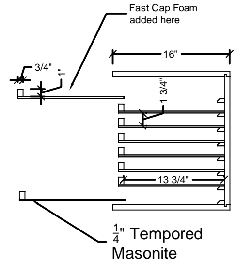
SECTION B 1 1/2" = 1'-0"
